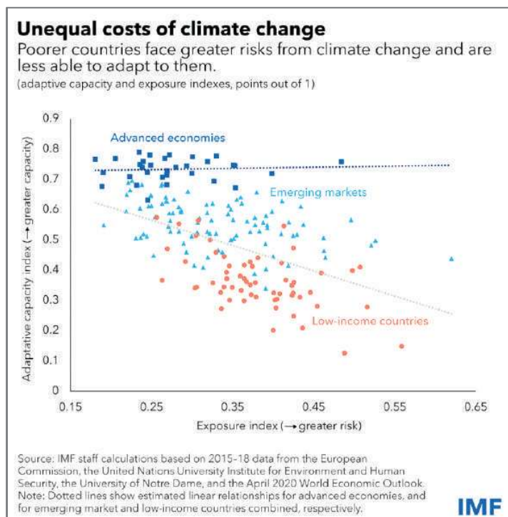
Figure 5: Unequal Costs of Climate Change
