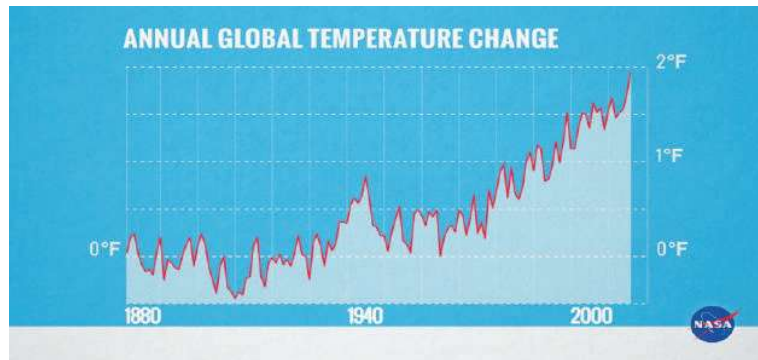
Figure 1: Change in Annual Global Temperatures, 1880-2016
